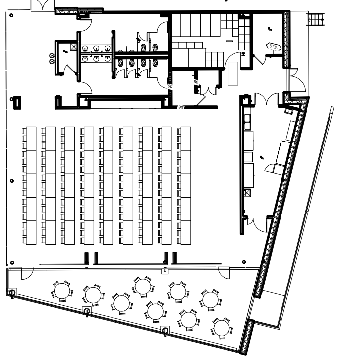
Conference Layout
